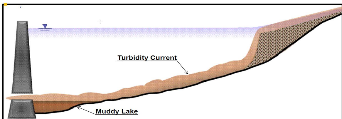
Figure 1: Release of turbid density current from reservoir
